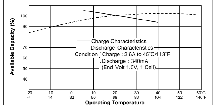
Temperature (Charge & Discharge)
