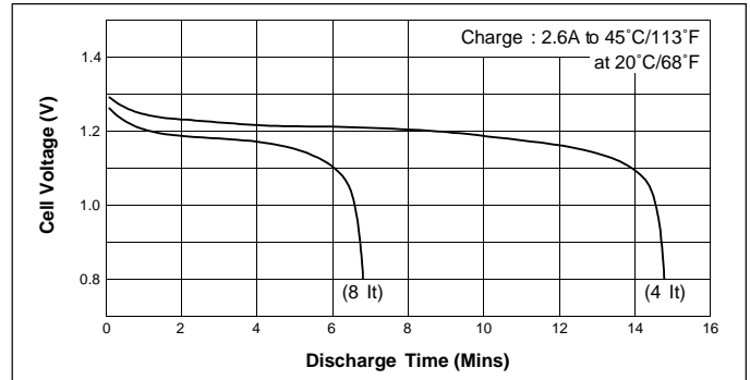
Discharge (high rate, 1 cell)
